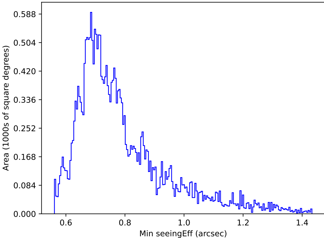
too_elab_r32_d2_gz_v3.4_10yrs Yr 1 g band: Min seeingEff
