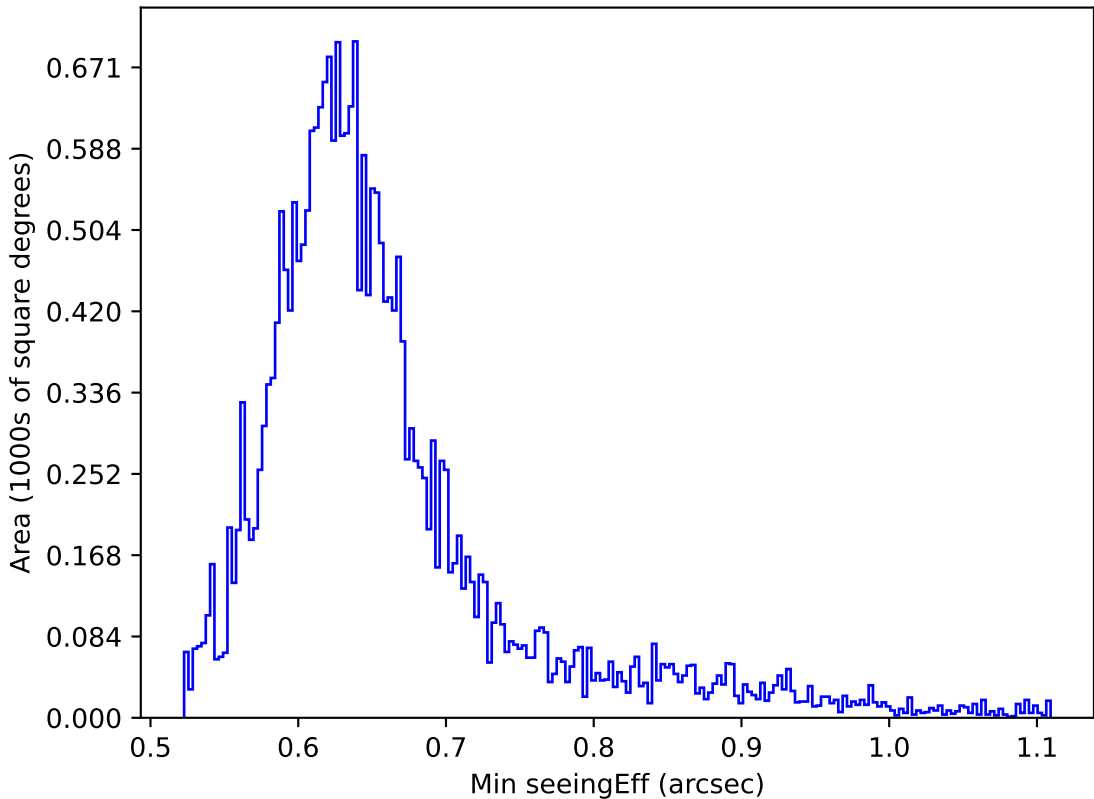
too_elab_r32_d2_gz_v3.4_10yrs Yr 1 all bands: Min seeingEff
