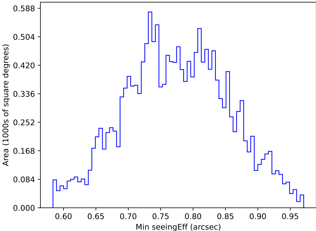
too_elab_r32_d2_gz_v3.4_10yrs WFD u band: Min seeingEff
