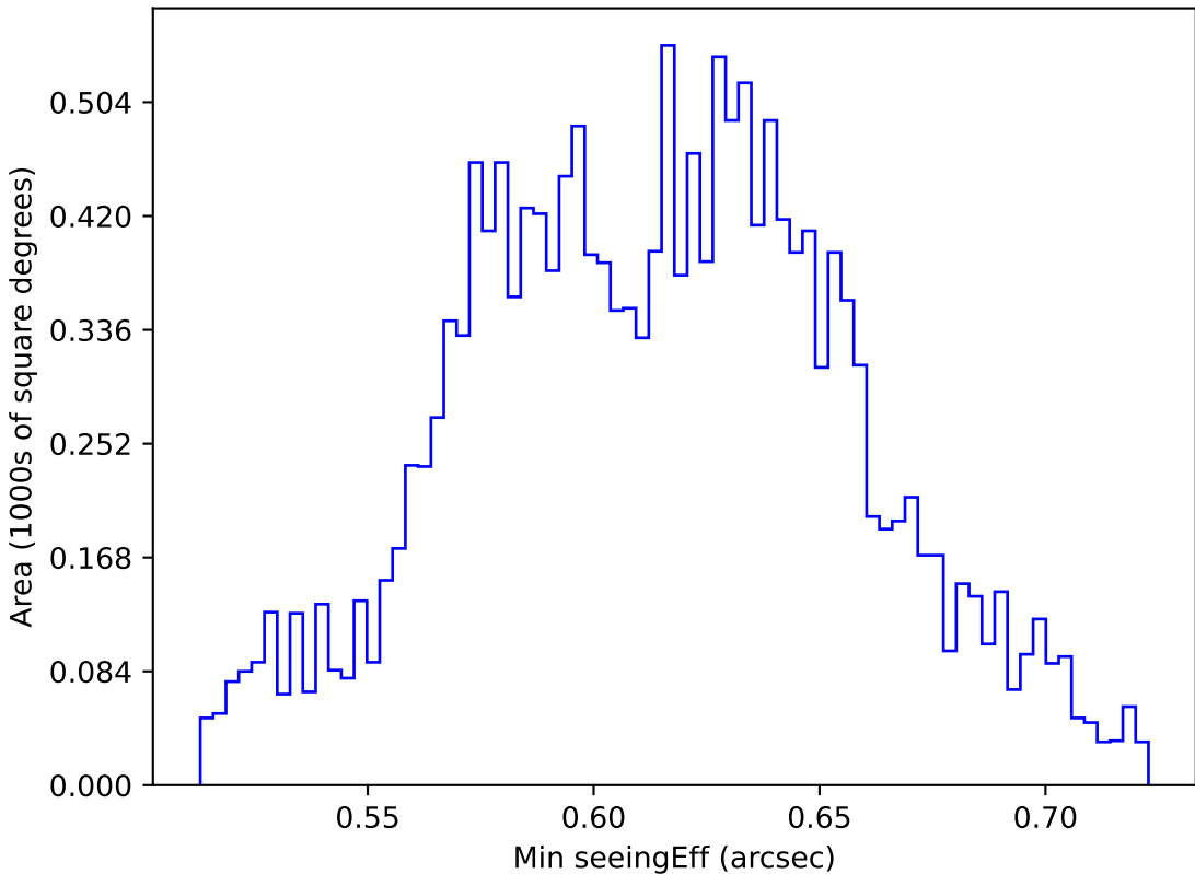
too_elab_r32_d2_gz_v3.4_10yrs WFD r band: Min seeingEff
