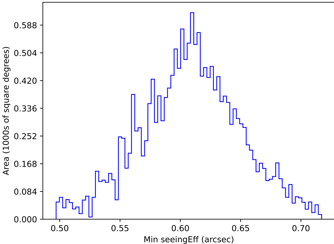
too_elab_r32_d2_gz_v3.4_10yrs WFD i band: Min seeingEff
