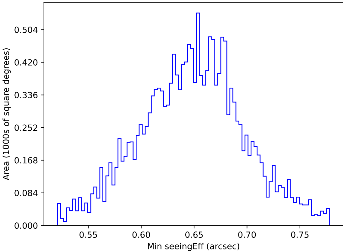
too_elab_r32_d2_gz_v3.4_10yrs WFD g band: Min seeingEff
