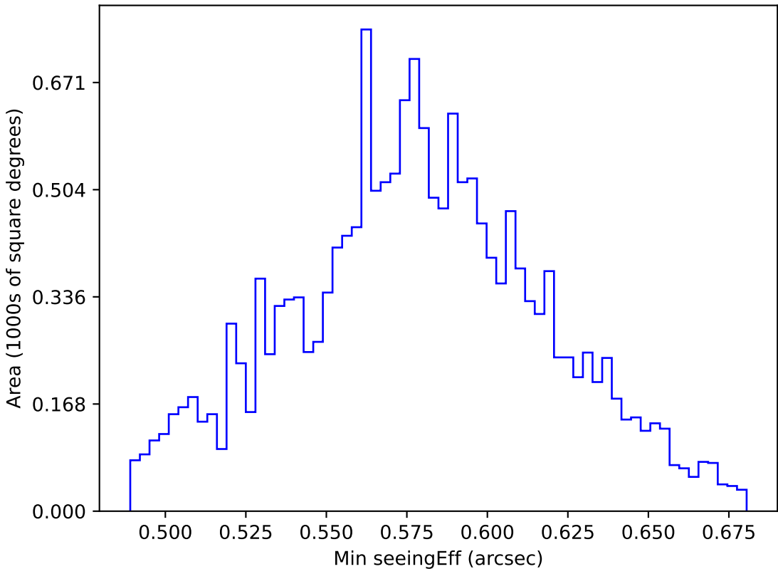
too_elab_r32_d2_gz_v3.4_10yrs WFD all bands: Min seeingEff
