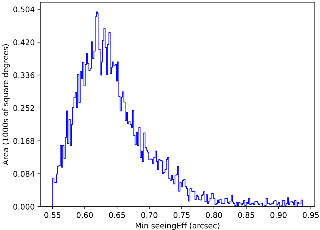
too_elab_r32_d2_gz_v3.4_10yrs All sky y band: Min seeingEff
