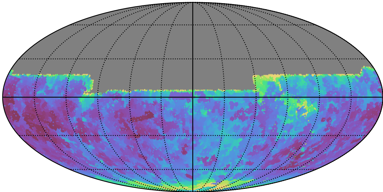
too_elab_r32_d2_gz_v3.4_10yrs All sky u band: Min seeingEff
