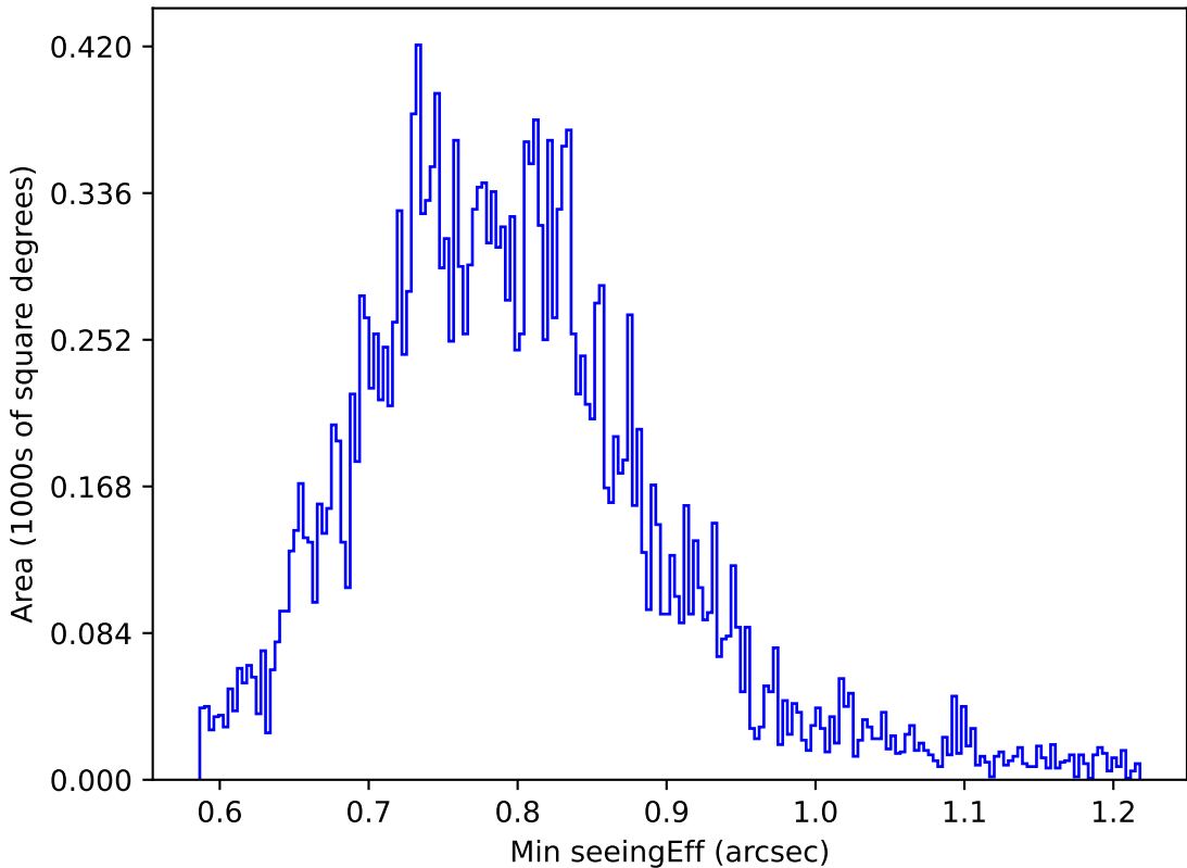
too_elab_r32_d2_gz_v3.4_10yrs All sky u band: Min seeingEff
