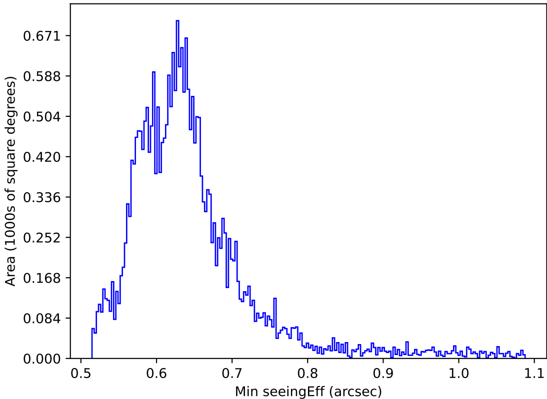
too_elab_r32_d2_gz_v3.4_10yrs All sky r band: Min seeingEff
