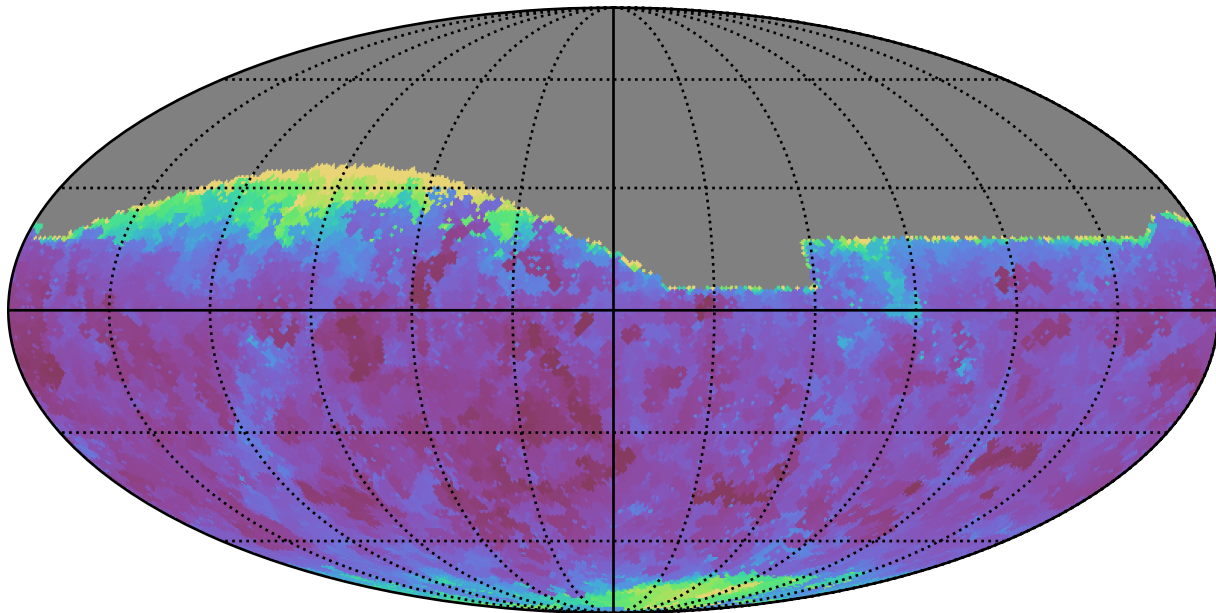
too_elab_r32_d2_gz_v3.4_10yrs All sky g band: Min seeingEff
