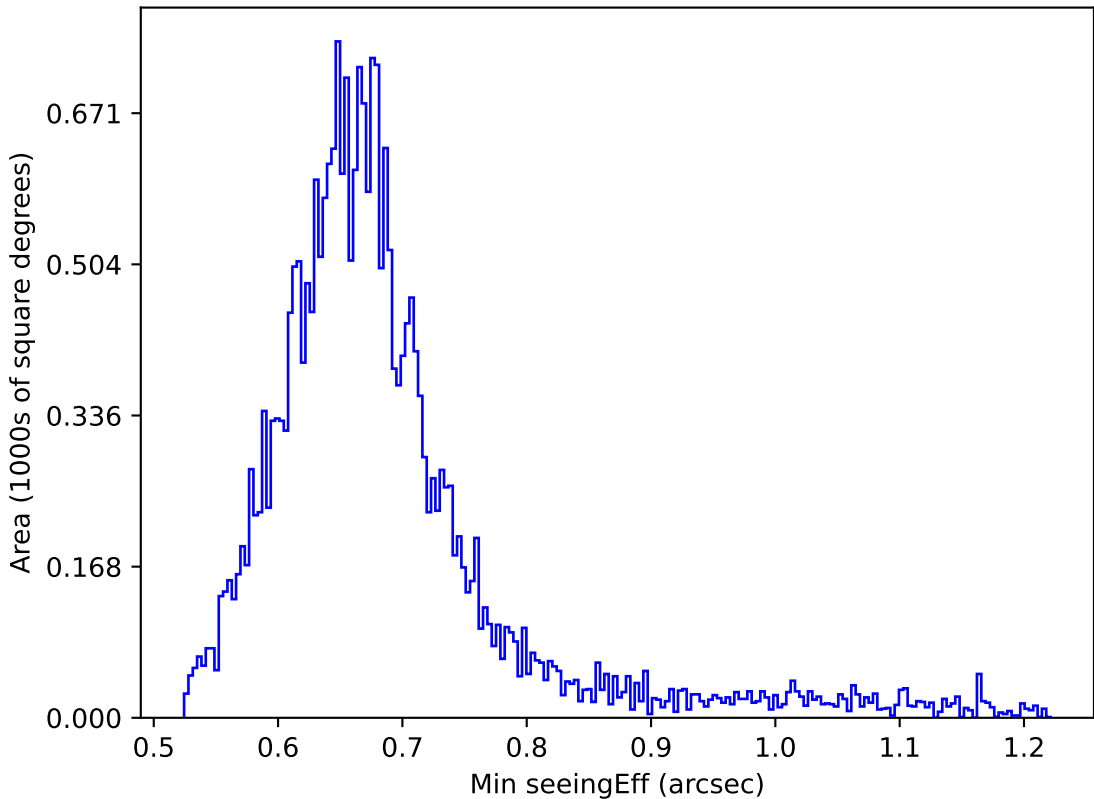
too_elab_r32_d2_gz_v3.4_10yrs All sky g band: Min seeingEff
