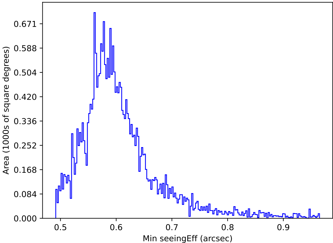
too_elab_r32_d2_gz_v3.4_10yrs All sky all bands: Min seeingEff
