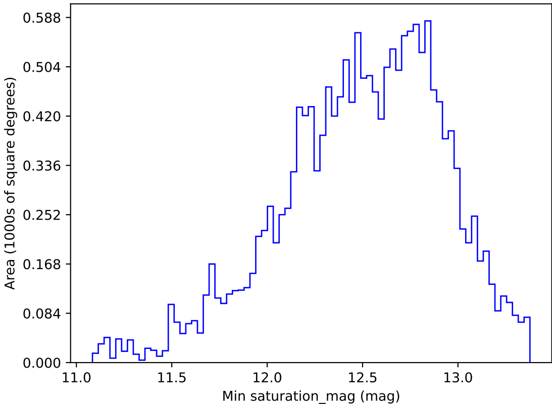
too_elab_r32_d2_gz_v3.4_10yrs WFD r band: Min saturation_mag
