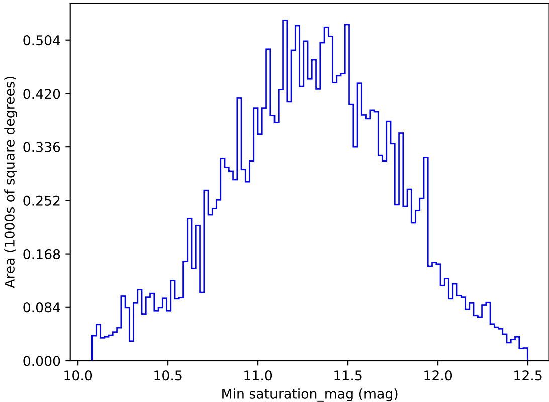
too_elab_r32_d2_gz_v3.4_10yrs All sky y band: Min saturation_mag
