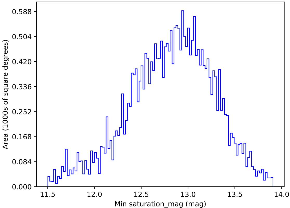
too_elab_r32_d2_gz_v3.4_10yrs All sky g band: Min saturation_mag
