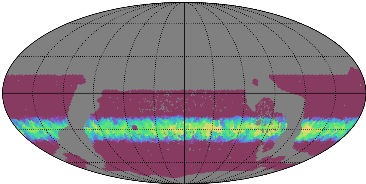
too_elab_r32_d2_gz_v3.4_10yrs WFD r band: Min normairmass
