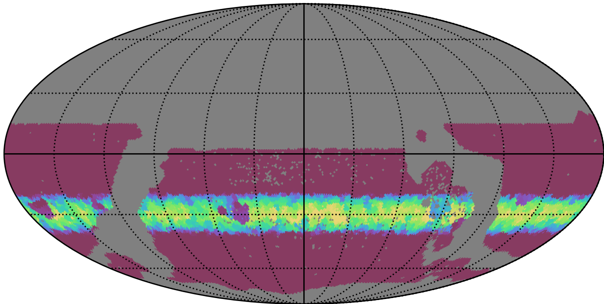
too_elab_r32_d2_gz_v3.4_10yrs WFD all bands: Min normairmass
