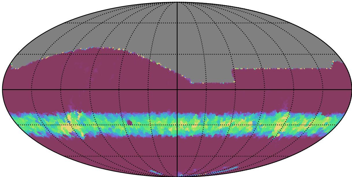
too_elab_r32_d2_gz_v3.4_10yrs All sky i band: Min normairmass
