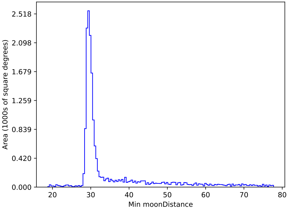
too_elab_r32_d2_gz_v3.4_10yrs WFD z band: Min moonDistance
