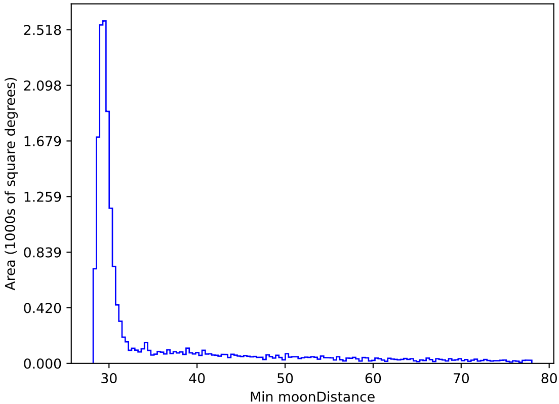
too_elab_r32_d2_gz_v3.4_10yrs WFD y band: Min moonDistance
