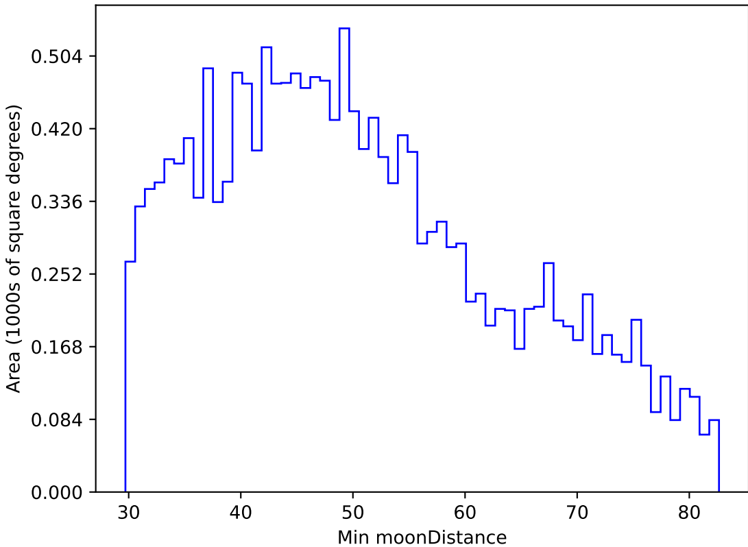
too_elab_r32_d2_gz_v3.4_10yrs WFD u band: Min moonDistance
