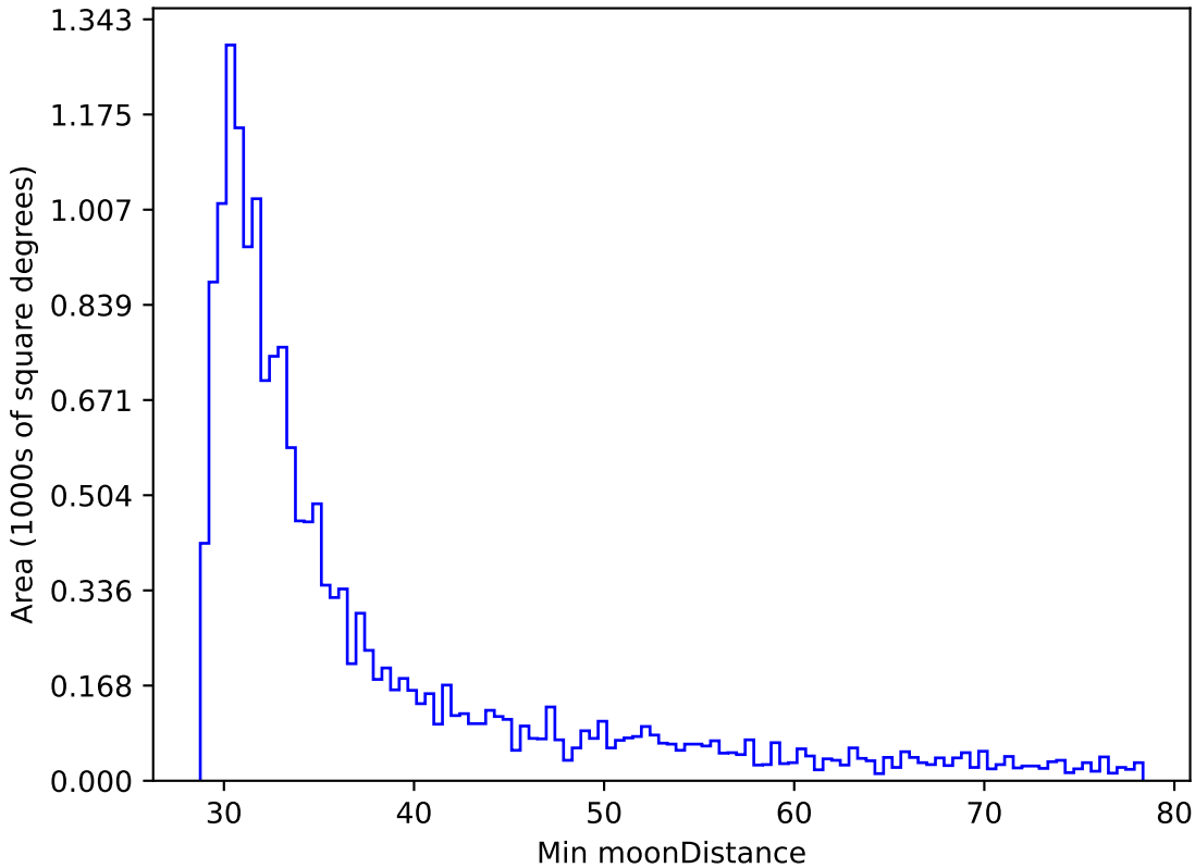
too_elab_r32_d2_gz_v3.4_10yrs WFD r band: Min moonDistance
