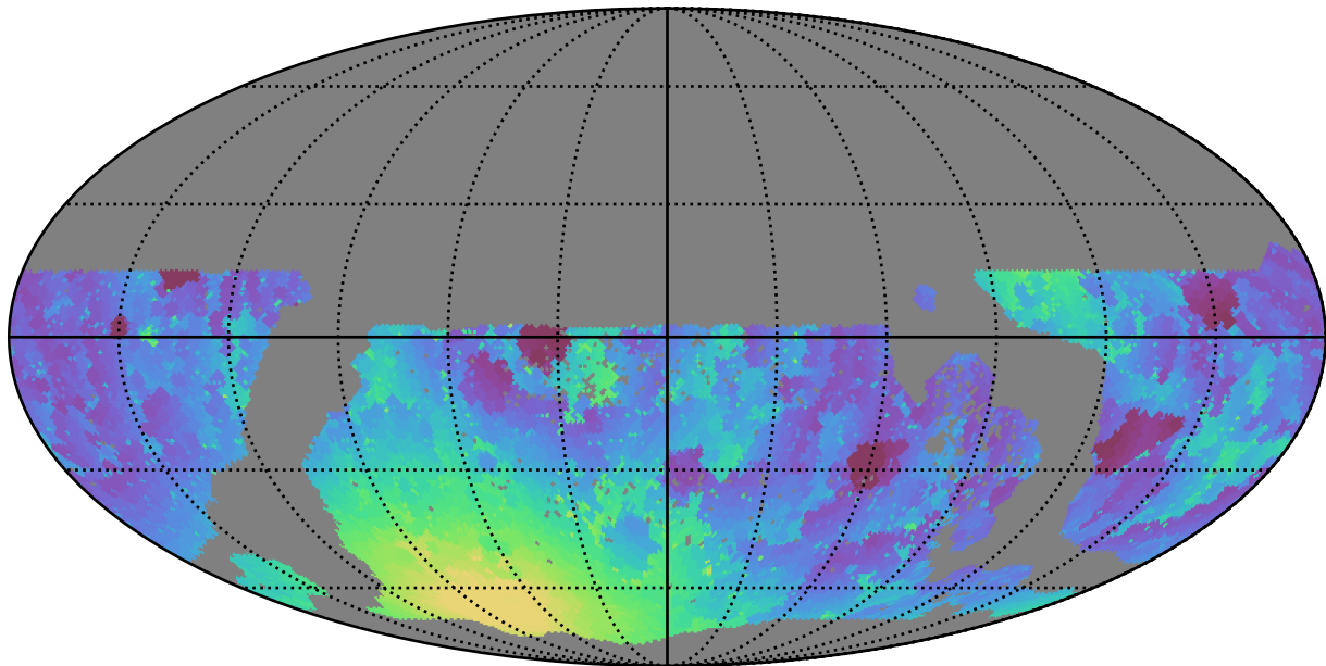
too_elab_r32_d2_gz_v3.4_10yrs WFD g band: Min moonDistance
