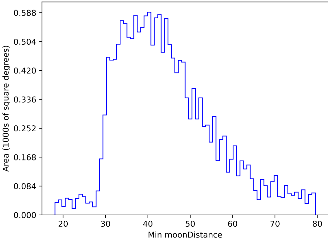
too_elab_r32_d2_gz_v3.4_10yrs WFD g band: Min moonDistance
