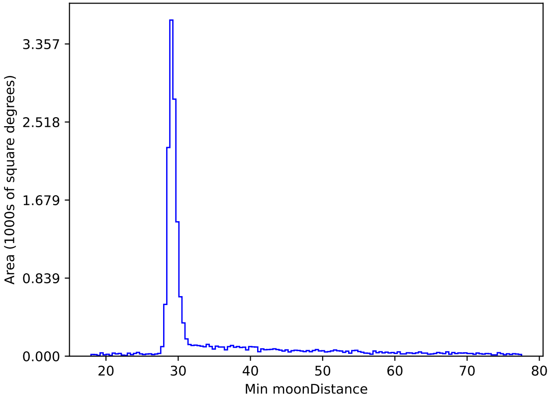
too_elab_r32_d2_gz_v3.4_10yrs WFD all bands: Min moonDistance
