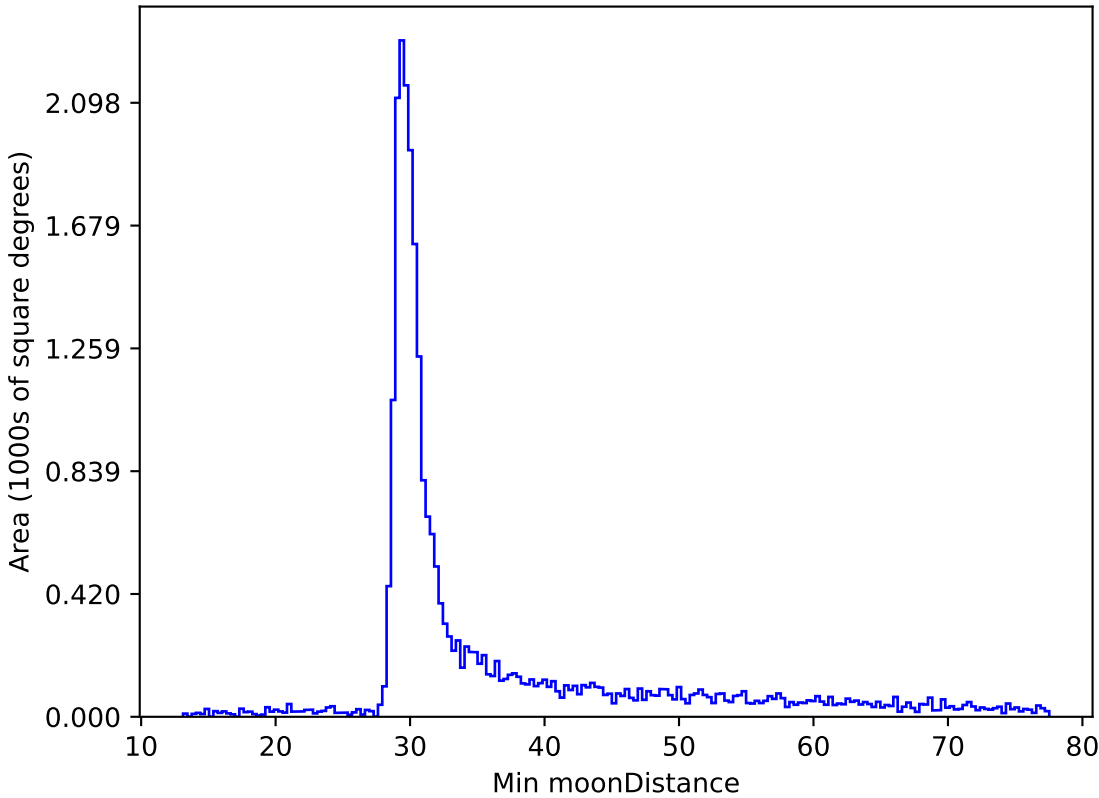
too_elab_r32_d2_gz_v3.4_10yrs All sky z band: Min moonDistance
