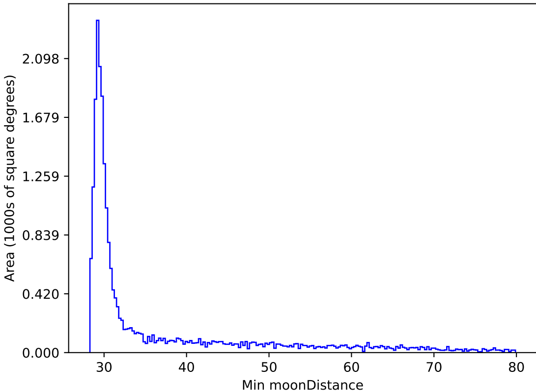
too_elab_r32_d2_gz_v3.4_10yrs All sky y band: Min moonDistance
