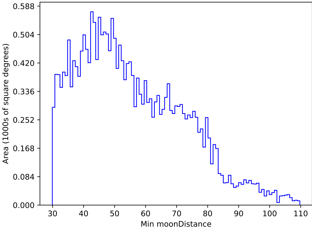
too_elab_r32_d2_gz_v3.4_10yrs All sky u band: Min moonDistance
