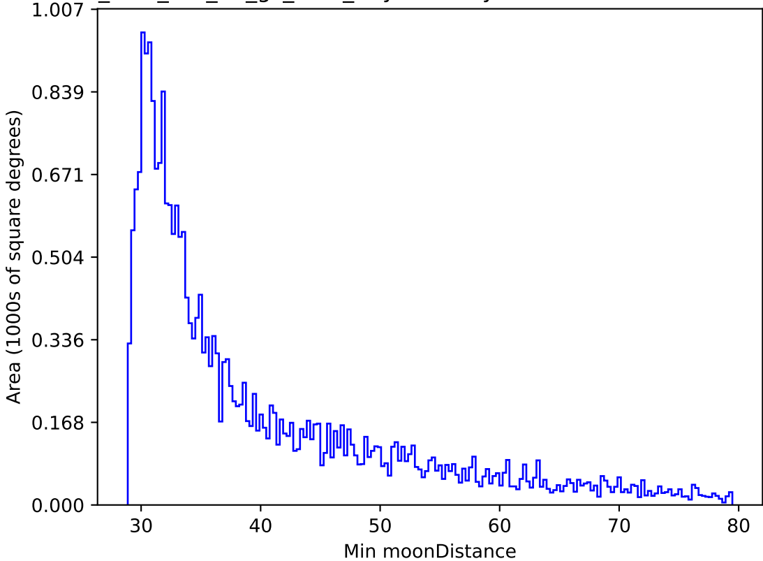
too_elab_r32_d2_gz_v3.4_10yrs All sky r band: Min moonDistance
