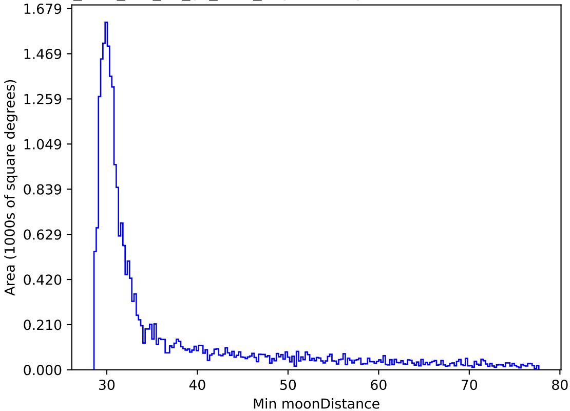
too_elab_r32_d2_gz_v3.4_10yrs All sky i band: Min moonDistance
