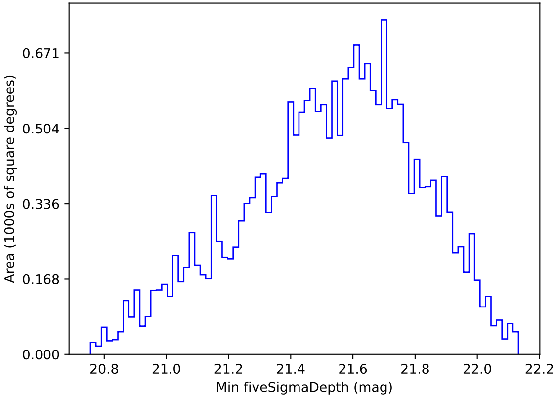
too_elab_r32_d2_gz_v3.4_10yrs Yr 1 y band: Min fiveSigmaDepth
