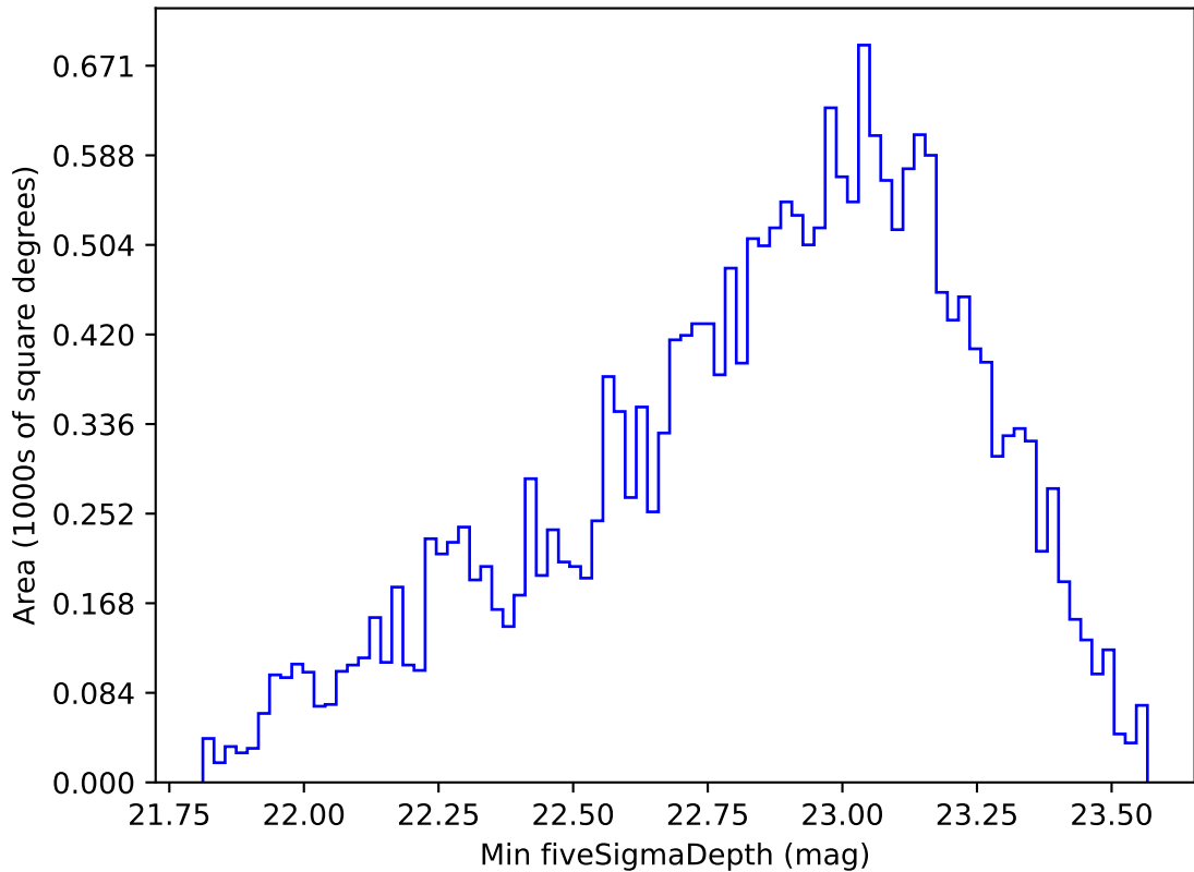
too_elab_r32_d2_gz_v3.4_10yrs Yr 1 u band: Min fiveSigmaDepth
