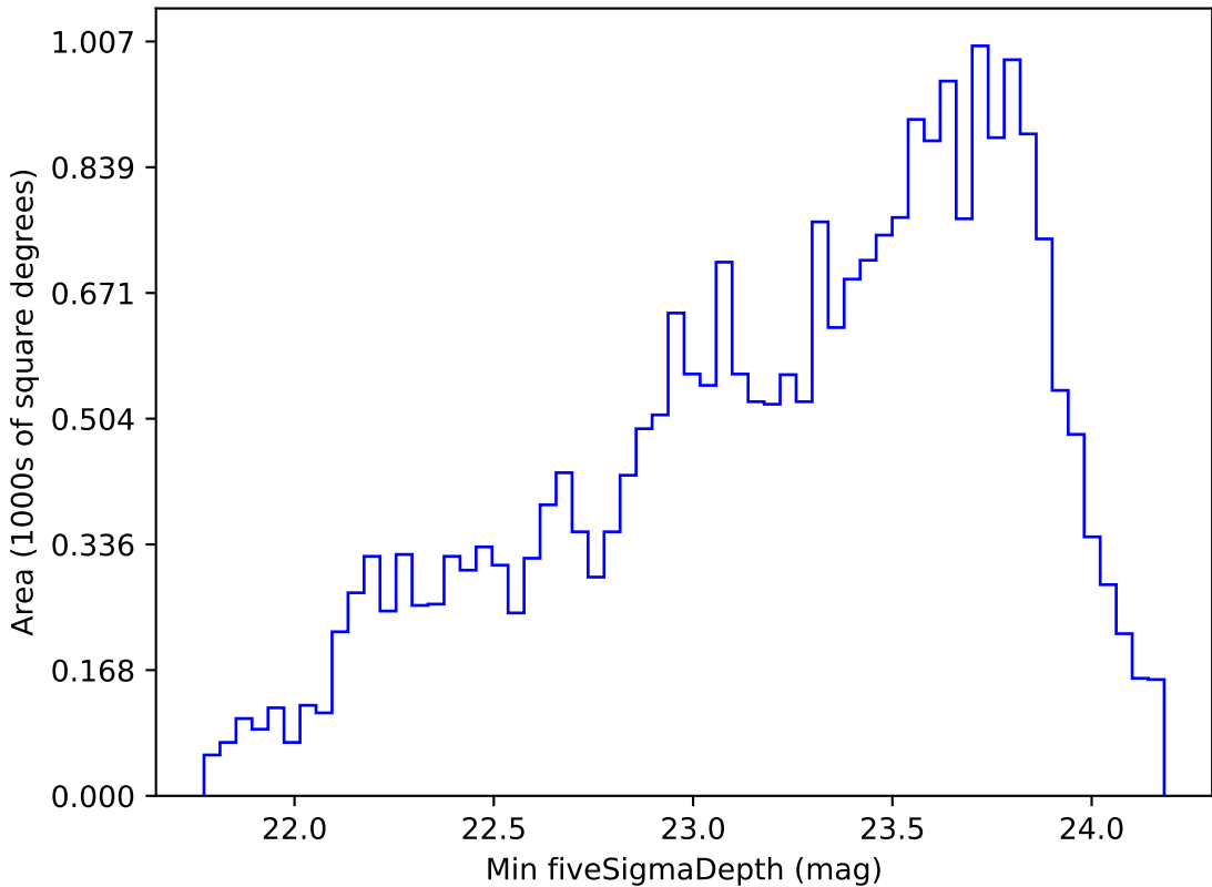
too_elab_r32_d2_gz_v3.4_10yrs Yr 1 r band: Min fiveSigmaDepth
