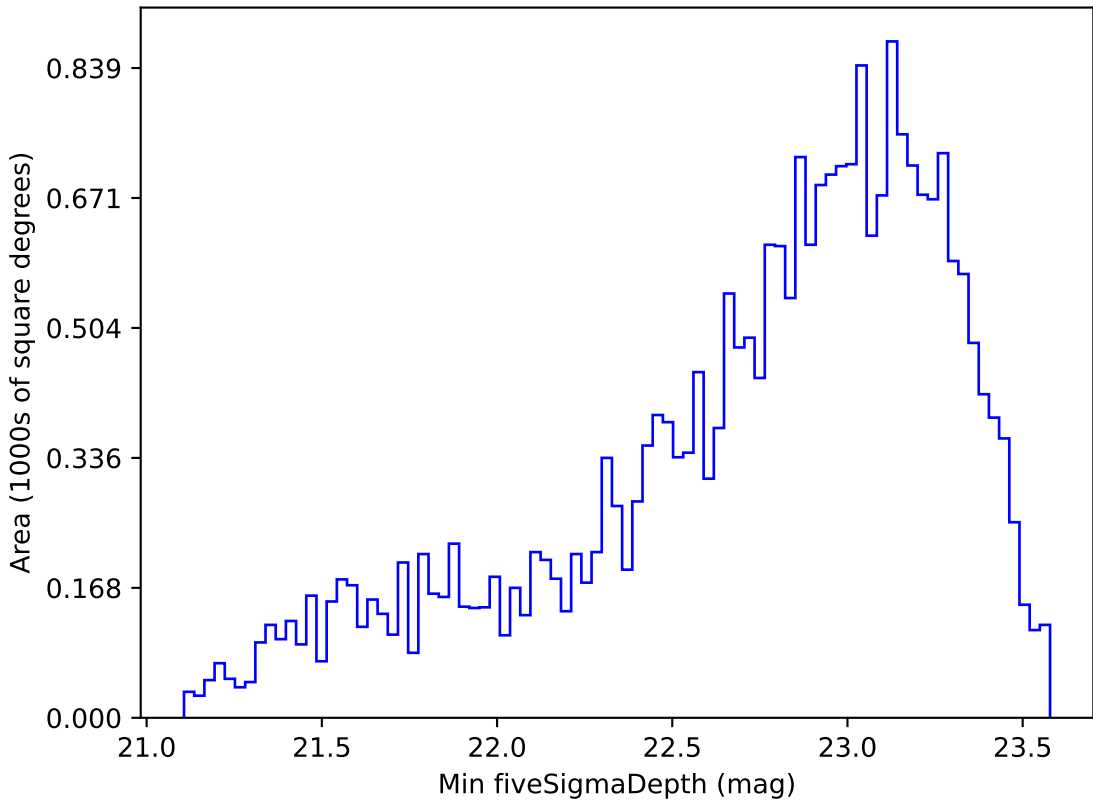
too_elab_r32_d2_gz_v3.4_10yrs Yr 1 i band: Min fiveSigmaDepth
