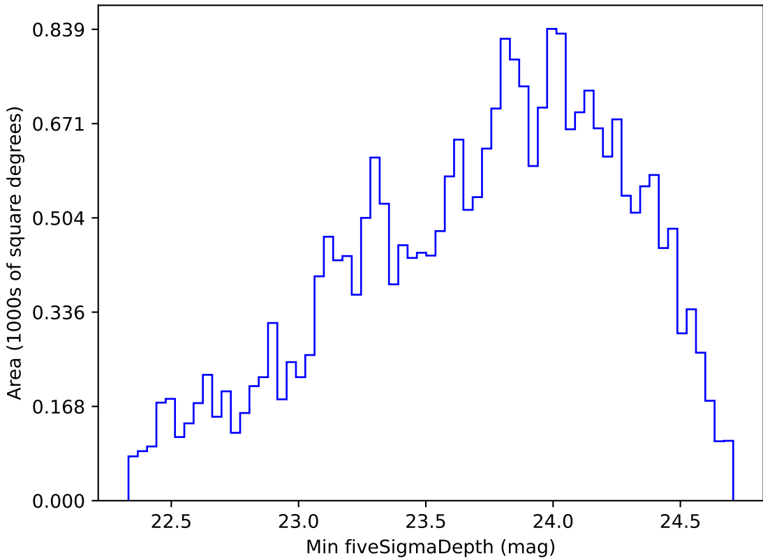
too_elab_r32_d2_gz_v3.4_10yrs Yr 1 g band: Min fiveSigmaDepth
