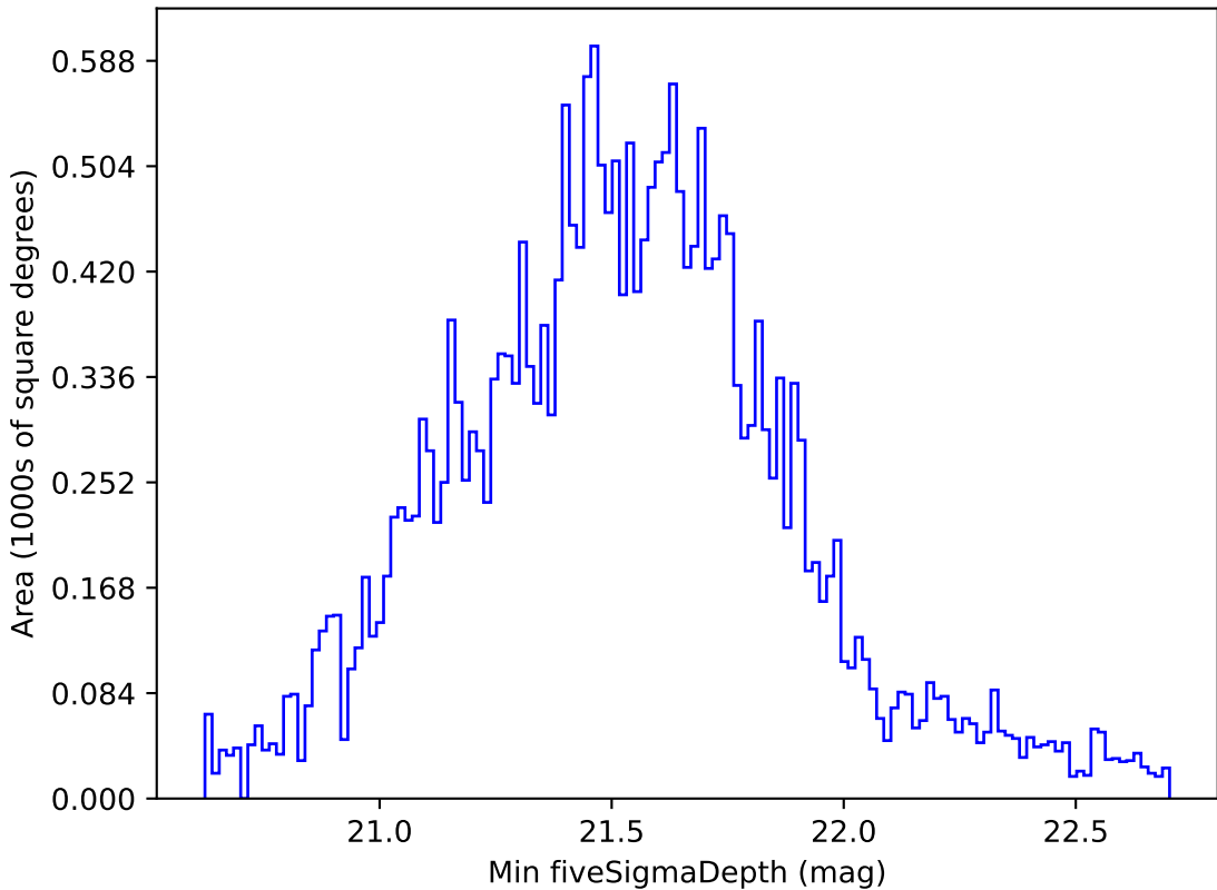
too_elab_r32_d2_gz_v3.4_10yrs Yr 1 all bands: Min fiveSigmaDepth
