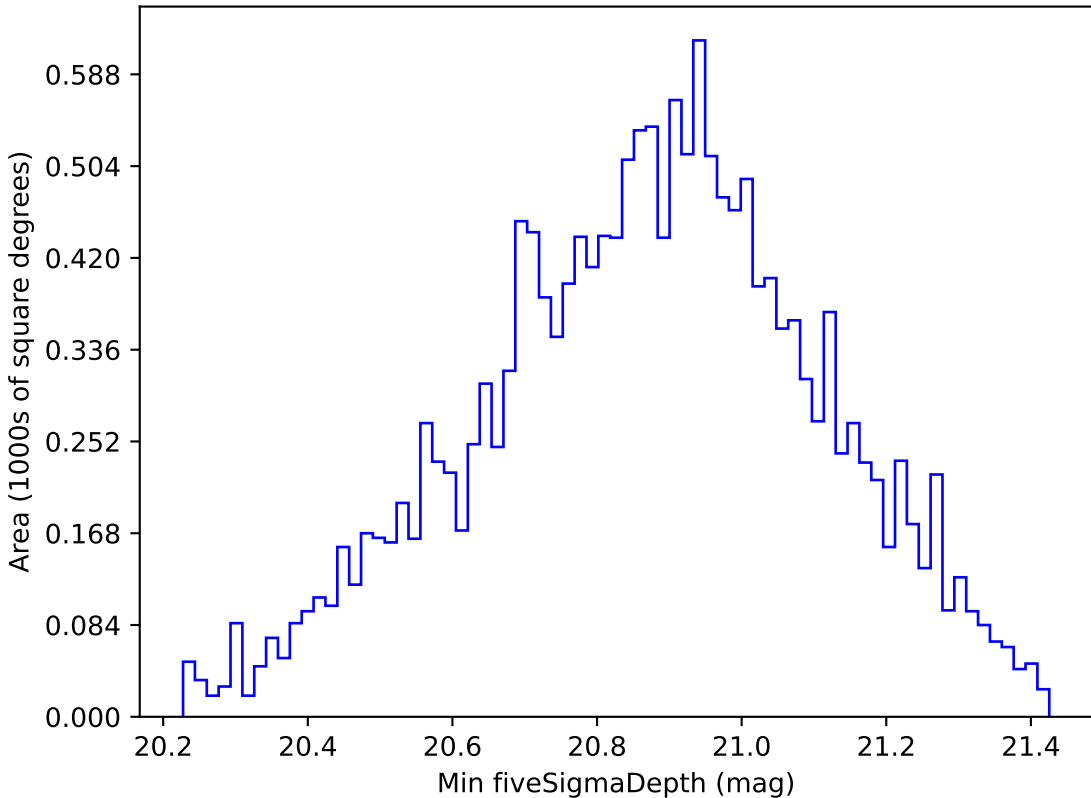
too_elab_r32_d2_gz_v3.4_10yrs WFD y band: Min fiveSigmaDepth
