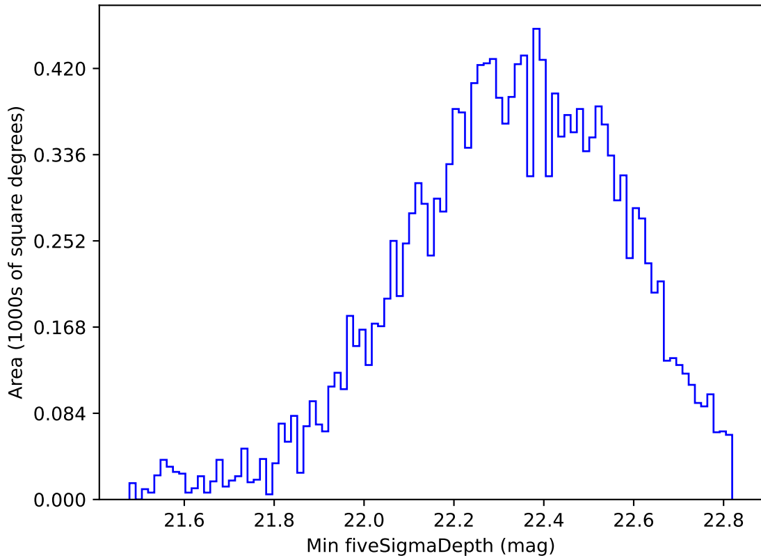
too_elab_r32_d2_gz_v3.4_10yrs WFD u band: Min fiveSigmaDepth
