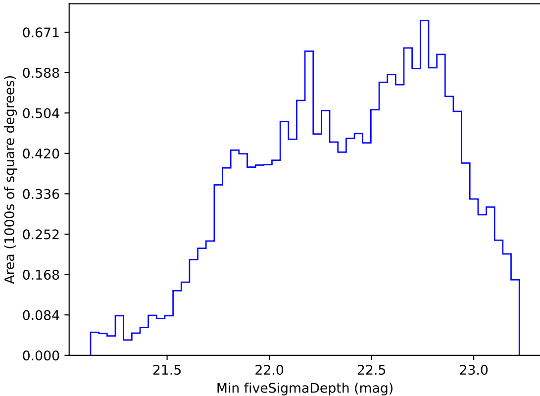
too_elab_r32_d2_gz_v3.4_10yrs WFD r band: Min fiveSigmaDepth
