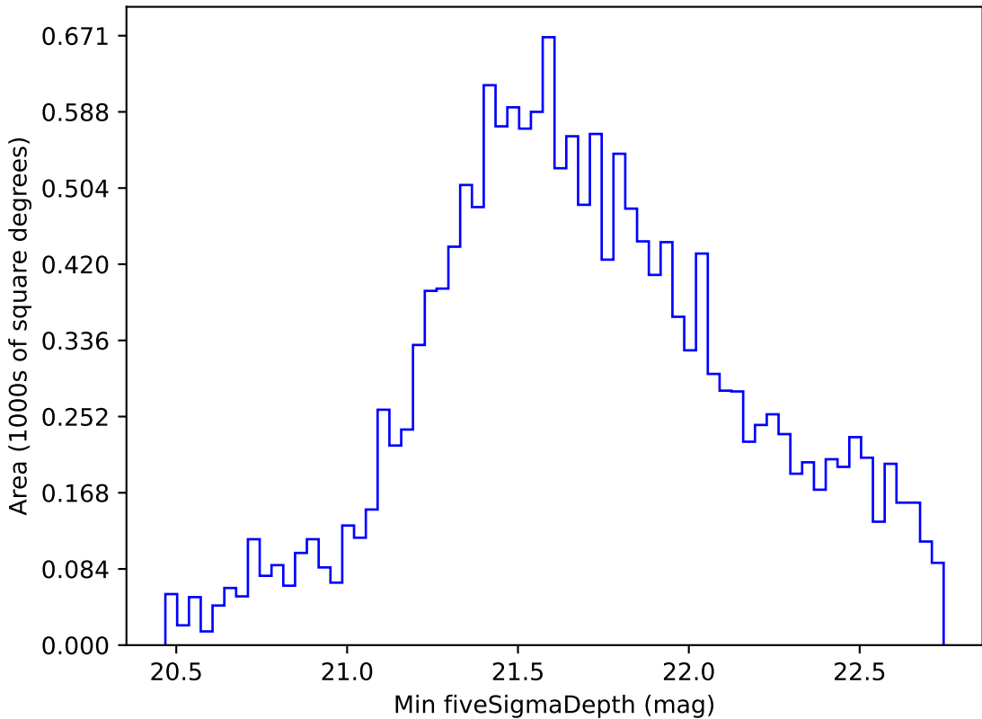
too_elab_r32_d2_gz_v3.4_10yrs WFD i band: Min fiveSigmaDepth
