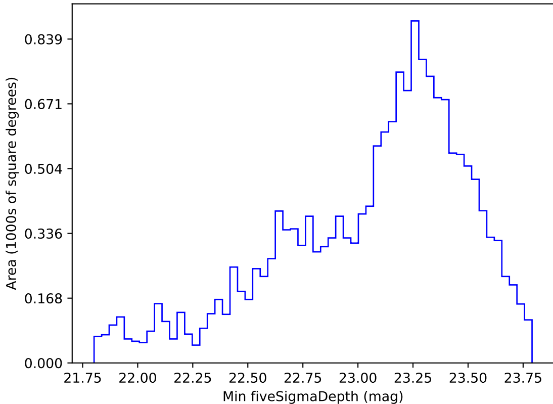
too_elab_r32_d2_gz_v3.4_10yrs WFD g band: Min fiveSigmaDepth
