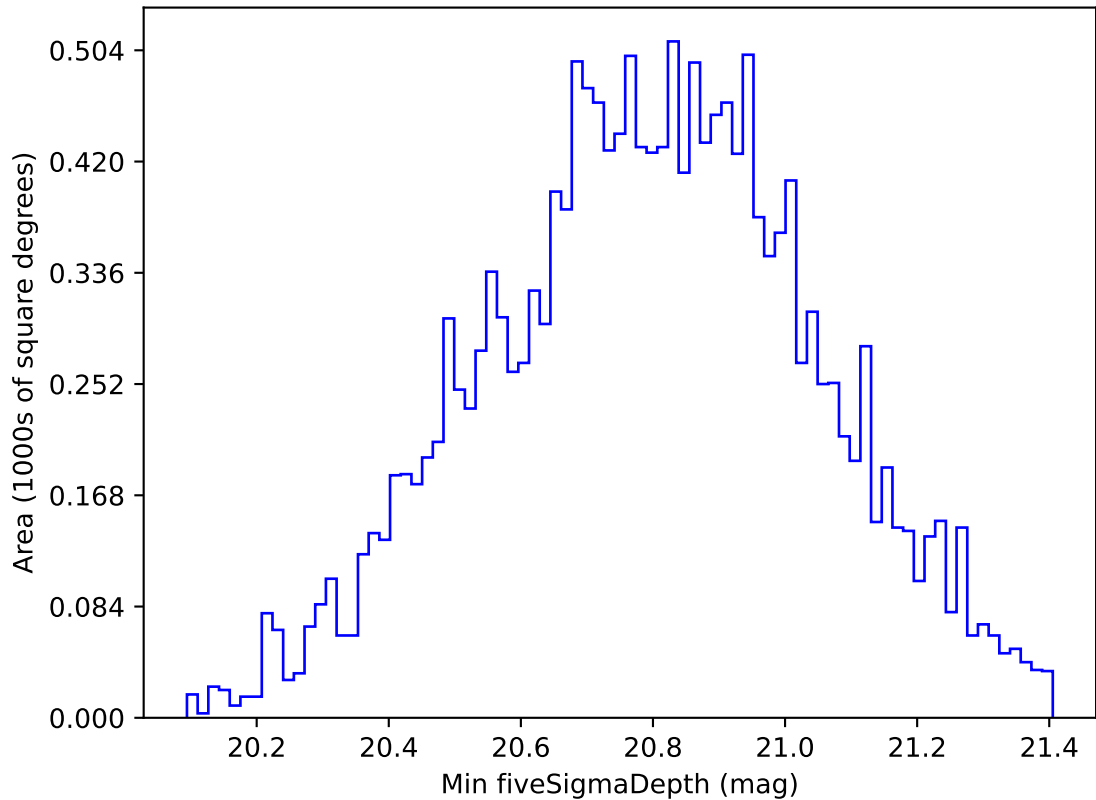
too_elab_r32_d2_gz_v3.4_10yrs WFD all bands: Min fiveSigmaDepth
