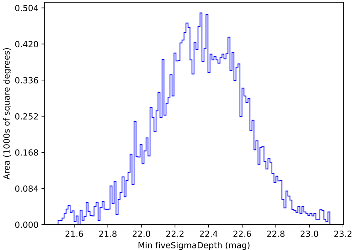
too_elab_r32_d2_gz_v3.4_10yrs All sky u band: Min fiveSigmaDepth
