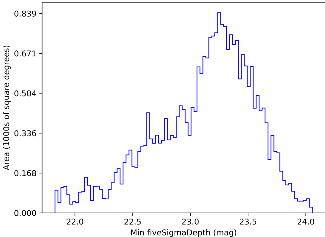
too_elab_r32_d2_gz_v3.4_10yrs All sky g band: Min fiveSigmaDepth
