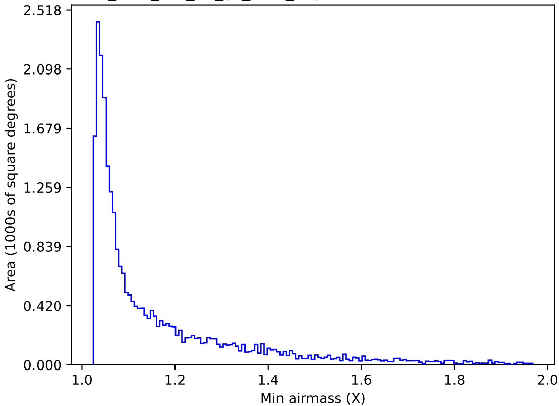
too_elab_r32_d2_gz_v3.4_10yrs Yr 1 z band: Min airmass
