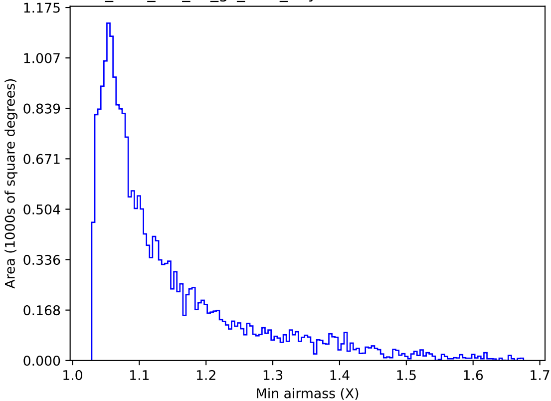
too_elab_r32_d2_gz_v3.4_10yrs Yr 1 u band: Min airmass
