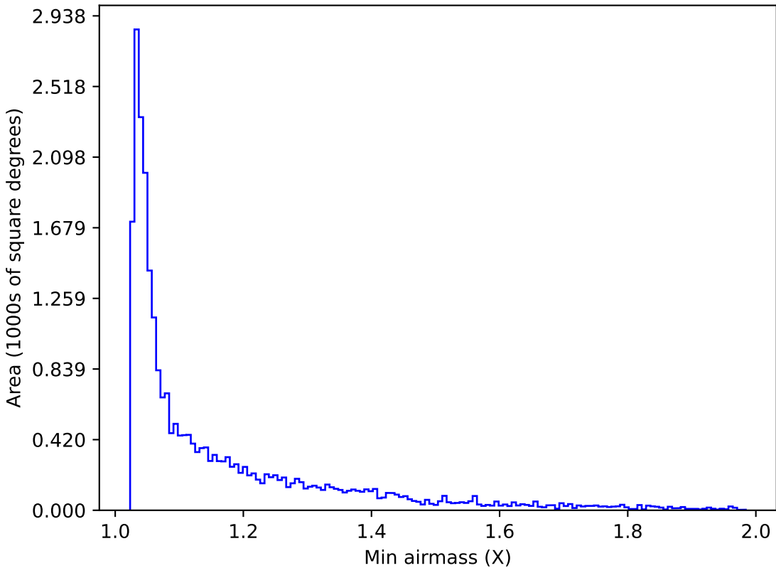
too_elab_r32_d2_gz_v3.4_10yrs Yr 1 r band: Min airmass
