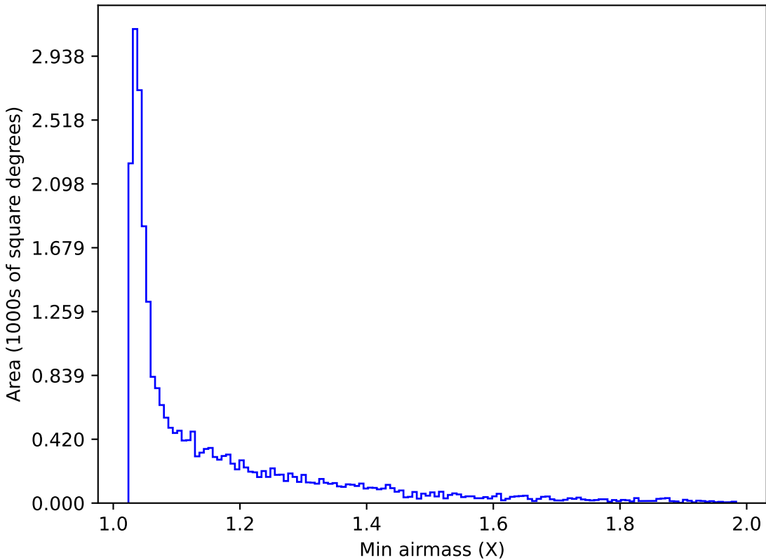
too_elab_r32_d2_gz_v3.4_10yrs Yr 1 i band: Min airmass
